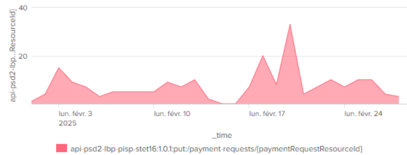
PISP - Nombre appels PUT /payment-requests/{id}
