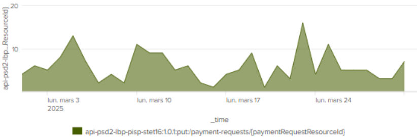
PISP - Nombre appels PUT /payment-requests/{id}
